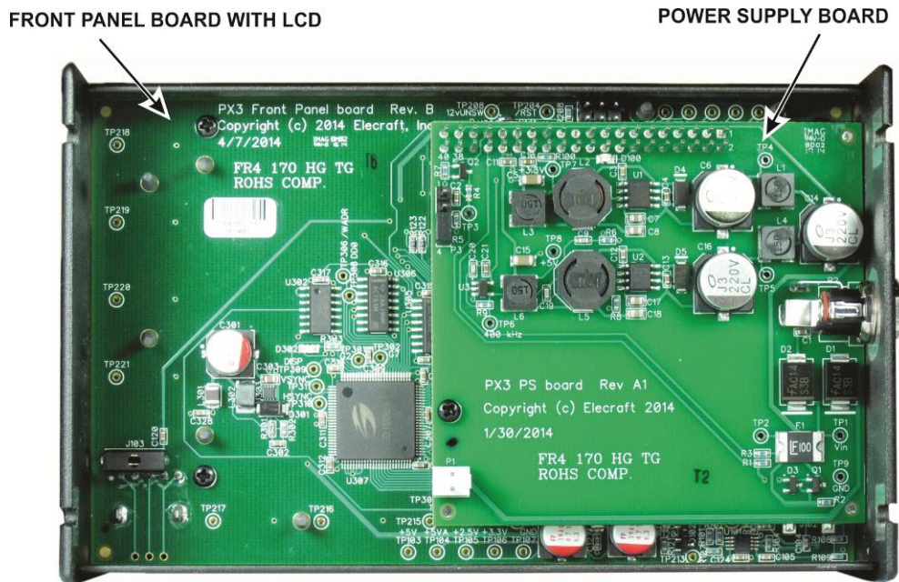
Figure 24 Assembled PX3 with Rear panel Removed.
