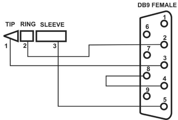
Figure 23. RS-232 Cable Schematic Diagram.
