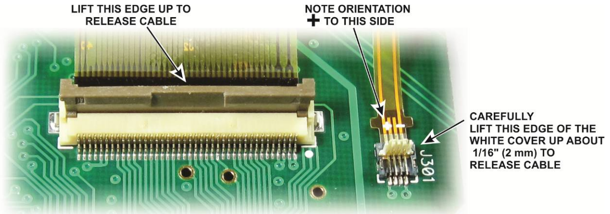
Figure 47. LCD Cable Connectors Opened.
