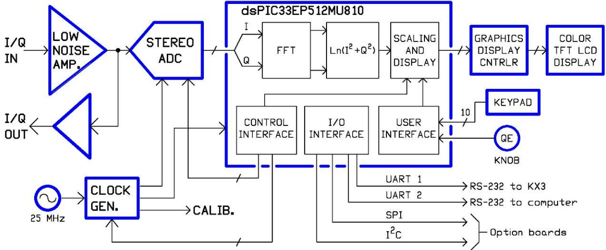
Figure 22. PX3 Simplified Block Diagram.
