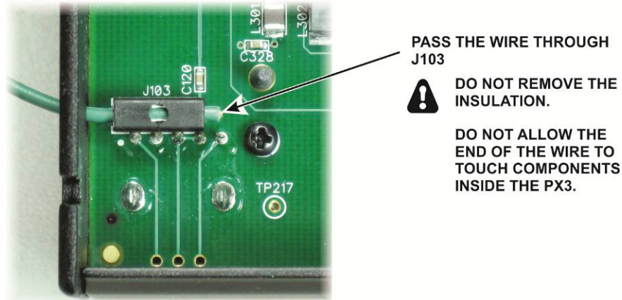
Figure 20. Calibrator Signal Pickup Wire Installed in the PX3.
