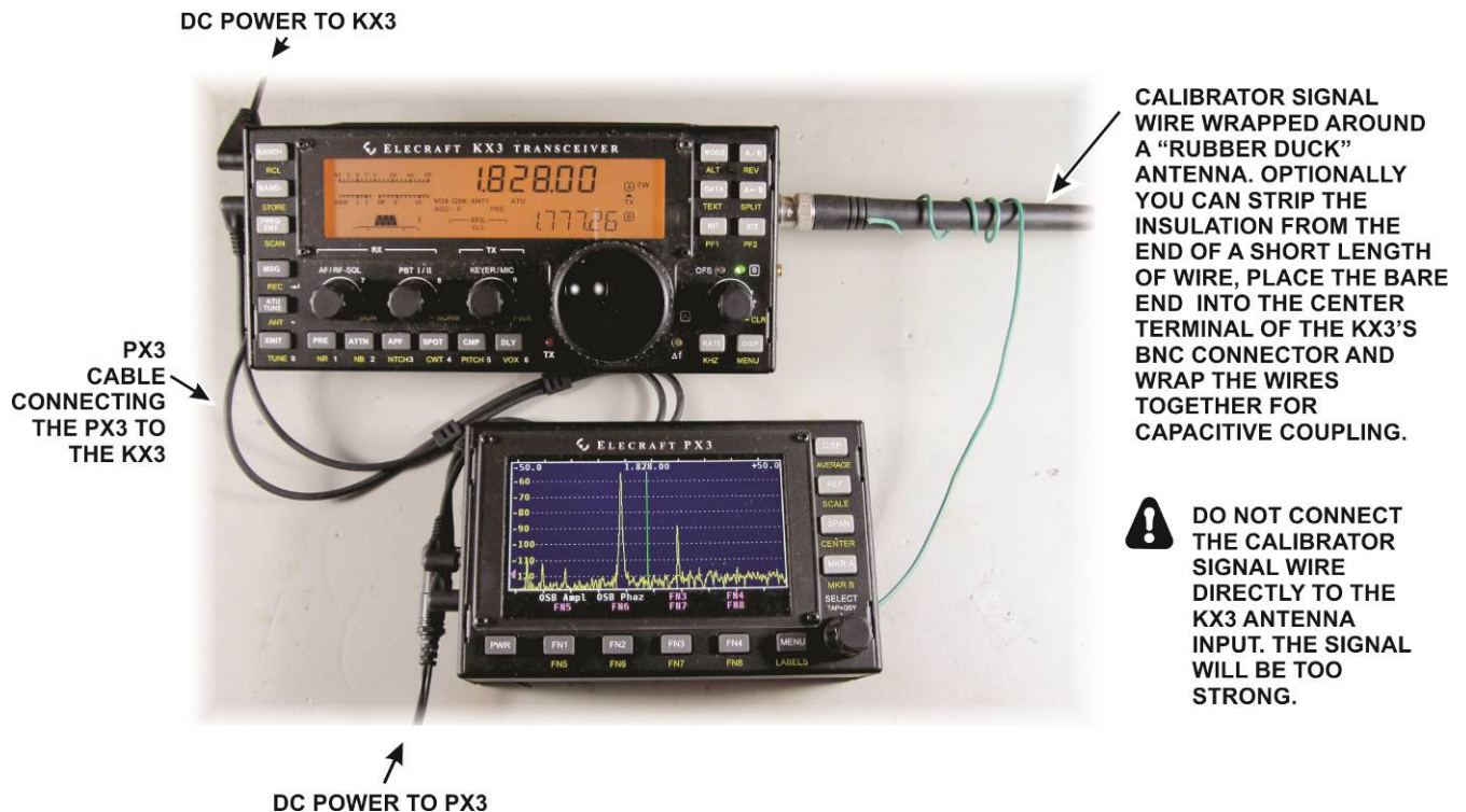
Figure 21. Opposite Sideband Nulling Setup Using Internal Signal Source.
