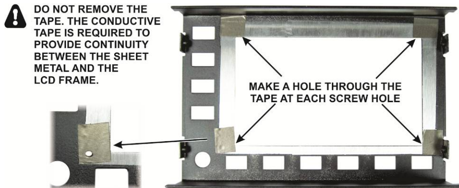
Figure 26. Front Panel Conductive Tape.
