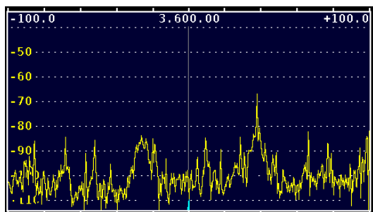
Figure 15. Typical Interference Display.
