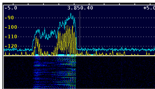
Figure 17. Typical SSB Spectra using Peak Hold.
