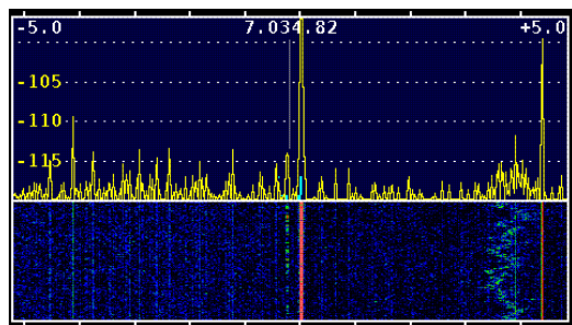
Figure 14. Typical Spectra Display.
