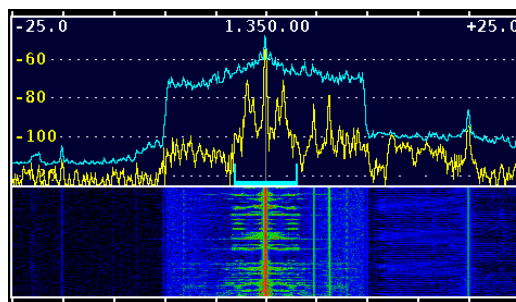
Figure 16. Typical AM Spectra using Peak Hold.
