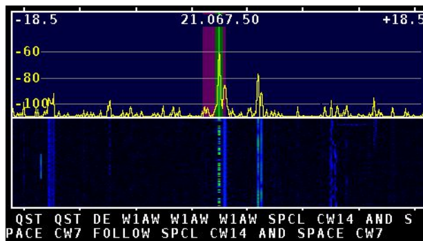
Figure 13. Decoded Text Display.
