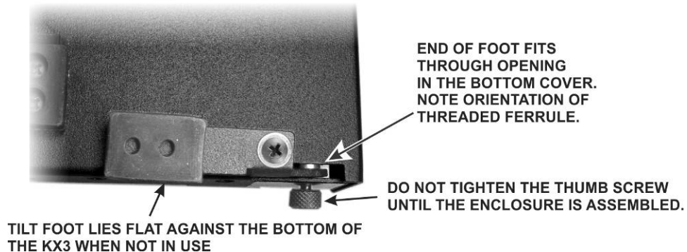
Figure 44. Installing the Tilt Feet in the Rear Cover.
