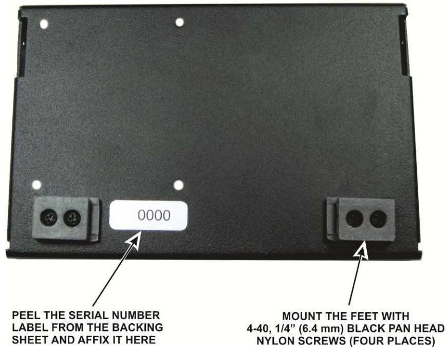
Figure 43. Installing Fixed Feet and Serial Number on the Rear panel.
